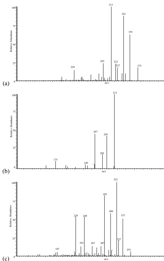
Figure 2. Examples of ESI-MS 3 and ESI-MS 4 spectra of salvinorin A: (a) MS 3 fragmentation of m/z 373 with 25% CE from ion m/z 433 with 20% CE; (b) MS 4 fragmentation of m/z 313 with 20% CE from m/z 433 (20% CE) and m/z 373 (25% CE); and (c) MS 4 fragmentation of m/z 355 with 30% CE from m/z 433 (20% CE) and m/z 373 (25% CE).
