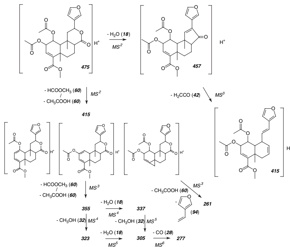
Scheme 2. Fragmentation pathways of salvinorin C.
