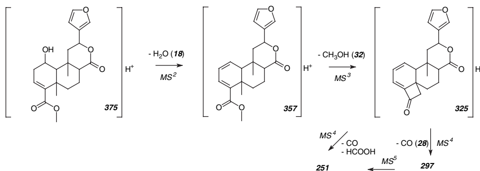
Scheme 3. Fragmentation pathways of salvinorin F.
