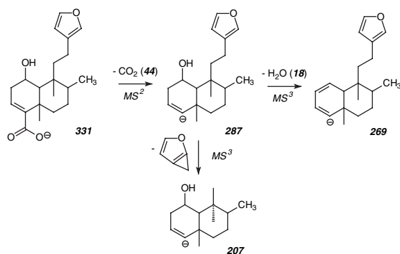
Scheme 4. Fragmentation pathways of divinatorin A.
