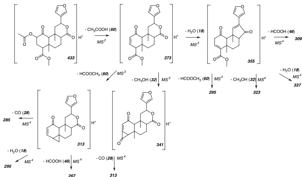
Scheme 1. Fragmentation pathways of salvinorin A.
