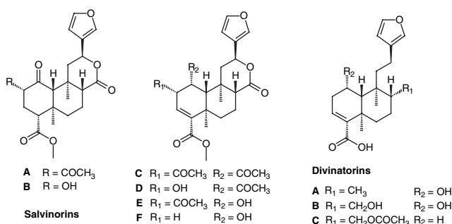
Figure 1. Structures of the six salvinorins and three divinatorins studied.
