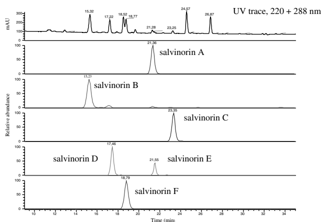
Figure 3. Chromatographic separation: trace 1: standard mixture of salvinorins and divinatorins, UV detection; trace 2: salvinorin A (MS 3 of m/z 373 with 25% CE from m/z 433 with 20% CE); trace 3: salvinorin B (MS 3 of m/z 373 with 27% CE from m/z 391 with 20% CE); trace 4: salvinorin C (MS 3 of m/z 415 with 30% CE from m/z 475 with 20% CE); trace 5: salvinorins D (first eluted) and E (MS 3 of m/z 415 with 30% CE from m/z 433 with 20% CE); trace 6: salvinorin F (MS 3 of m/z 357 with 27% CE from m/z 375 with 25% CE).
